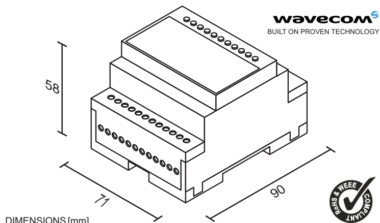
DIMENSIONS [mm]
